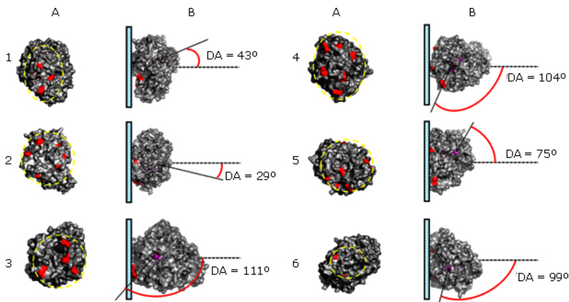
Fig. 3. Graphical representation of the different possible configurations of Trametes versicolor laccase-AuNP-MUA support system, predicted by RDID 1,0 software from the predicted clusters. (1-3) Clusters 1-3. (A) Possible clusters in laccase (surface representation) for covalent immobilization on AuNP-MUA support. (B) Most probable configuration of the immobilized derivative by each cluster. Grey: Enzyme surface area. Blue: Residues with amino groups on the enzyme surface. Discontinuous red circles: Cluster delimitation. DA: Deviation angle. Arrow: Active site entrance. Black discontinuous line: Normal of the nanoparticle surface.
