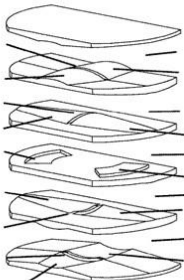
Fig. 7: Modular prosthesis for cervical and lumbar spine. United Kingdom. Patente n.º GB 2471133 A.
