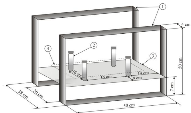
Figure 1a. The schematic representation of the experimental electromagnet setup (BioNak-03-1 electromagnet): (1) two parallel coils; (2) tubes with samples are placed inside of the air gap of coils (16 cm in distance from each other) to expose seedlings to electromagnetic field (60 Hz MF, 2mT during 3min); (3) tray; (4) horizontal plane of electromagnetic induction received by samples.
