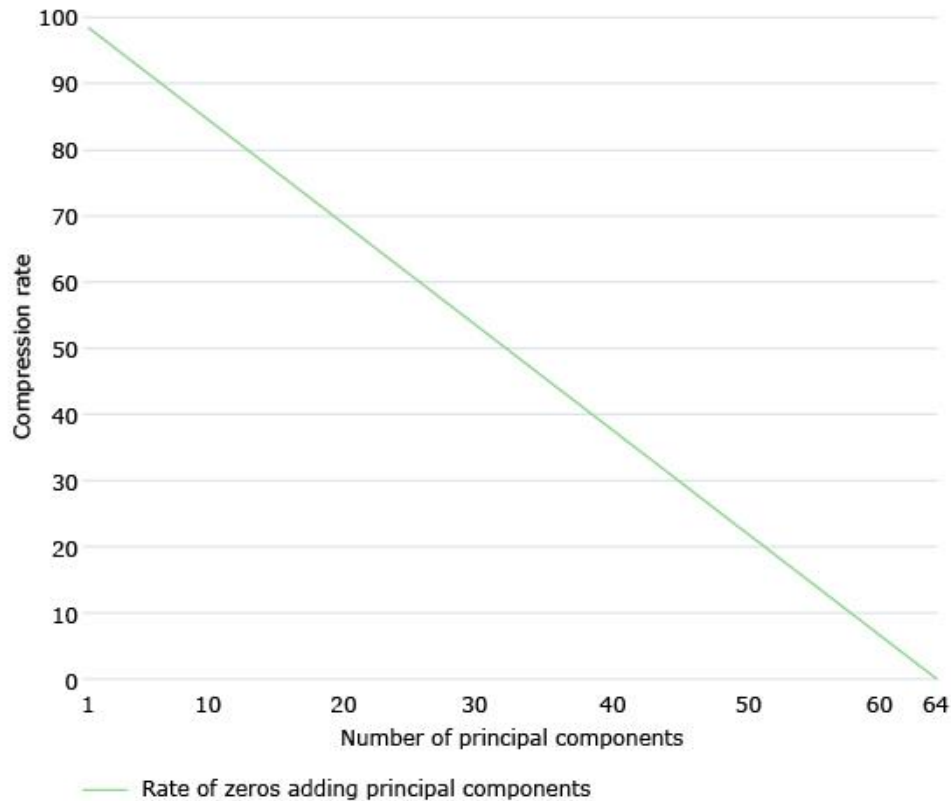
Fig. 5 - Compression rate of the original image as principal components are added.
