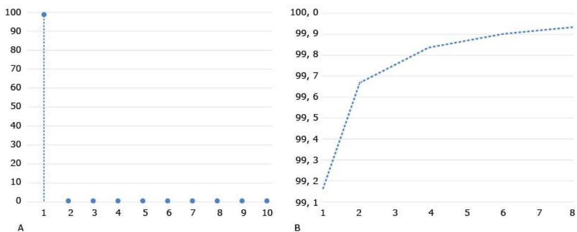
Fig. 3 - Magnitude of the first eigenvalues and explained accumulated variance. A. Magnitude ( \lambda_k ) of the first 10 eigenvalues ( k, k = 1 \dots 10 ); B. Cumulative variability ( I_k ) explained with the first 8 eigenvalues ( k, k = 1 \dots 8 ).
