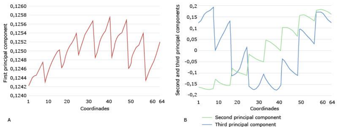
Fig. 7 - Graphs of the first three PCs of X 1 . A. First PC; B. Second and third PCs.
