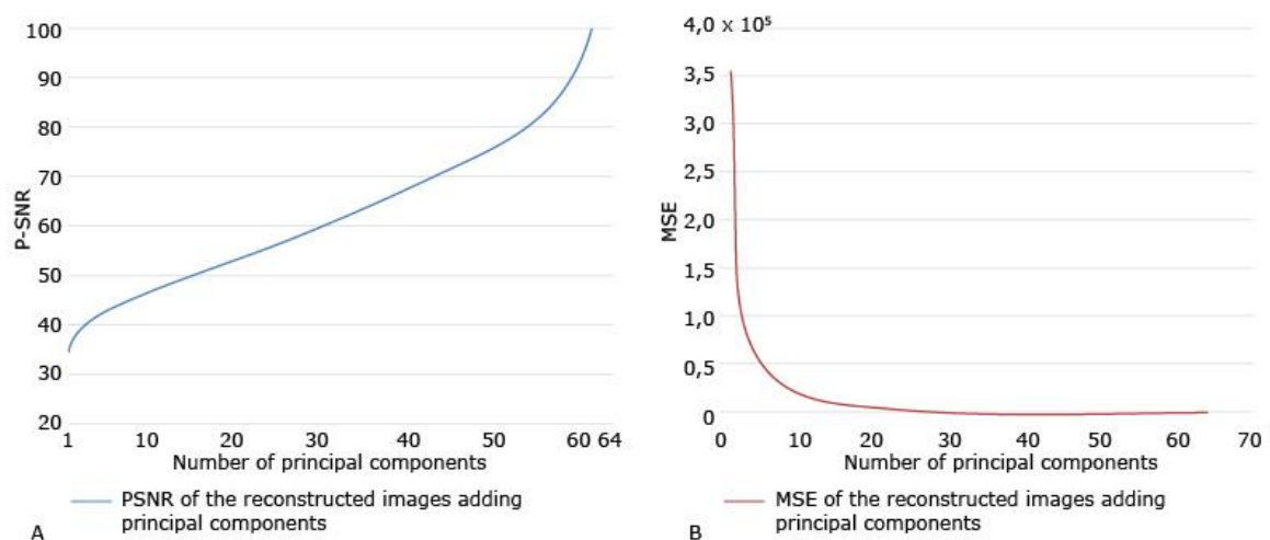
Fig. 4 - PSNR and MSE of the original image versus the compressed images as PCs are added to the compression. A. PSNR of the original image versus the compressed images; B. MSE of the original image versus the compressed images.
