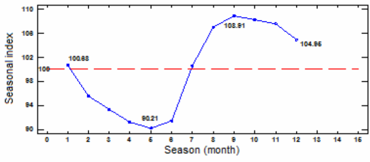
Fig. 1. Seasonability indexes for technical efficiency of artificial insemination
