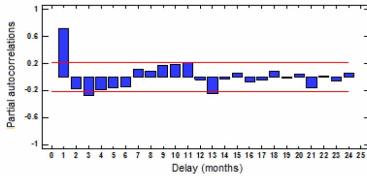
Fig. 2. Estimated partial autocorrelations for technical efficiency of artificial insemination
